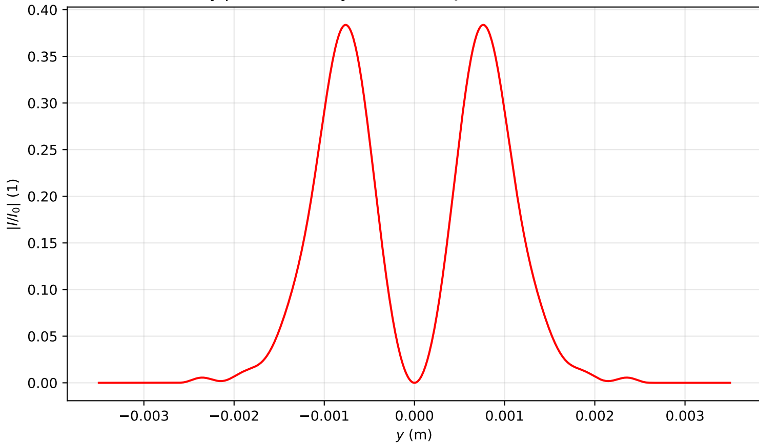
Intensity profile I(x=0, y, z=2.946)/I_0 , P_{in}=3.0P_{cr} , artificial time
